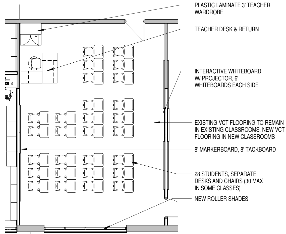
CLASSROOM LAYOUT A
